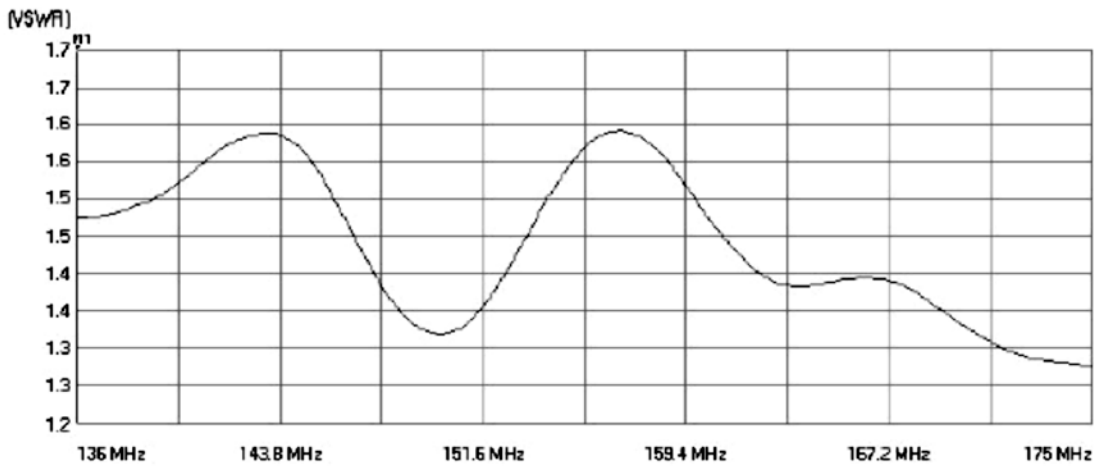
Rolatube 7m RESQ Integrated Antenna Mast (136 - 175 MHz) - VSWR Trace
